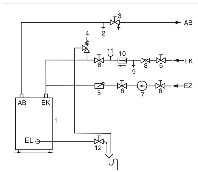
Fig. 6 Tank piping installation (sample picture)
