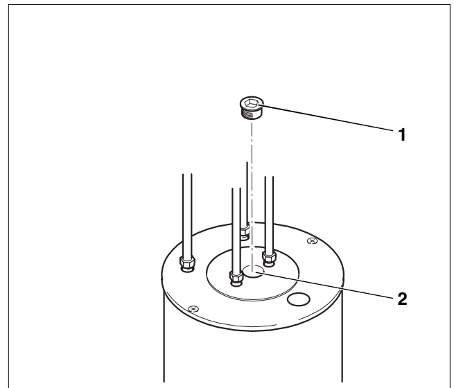
Fig. 11 Removal of inspection plug
