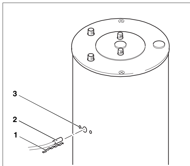
Fig. 7 Installation of temperature sensor
