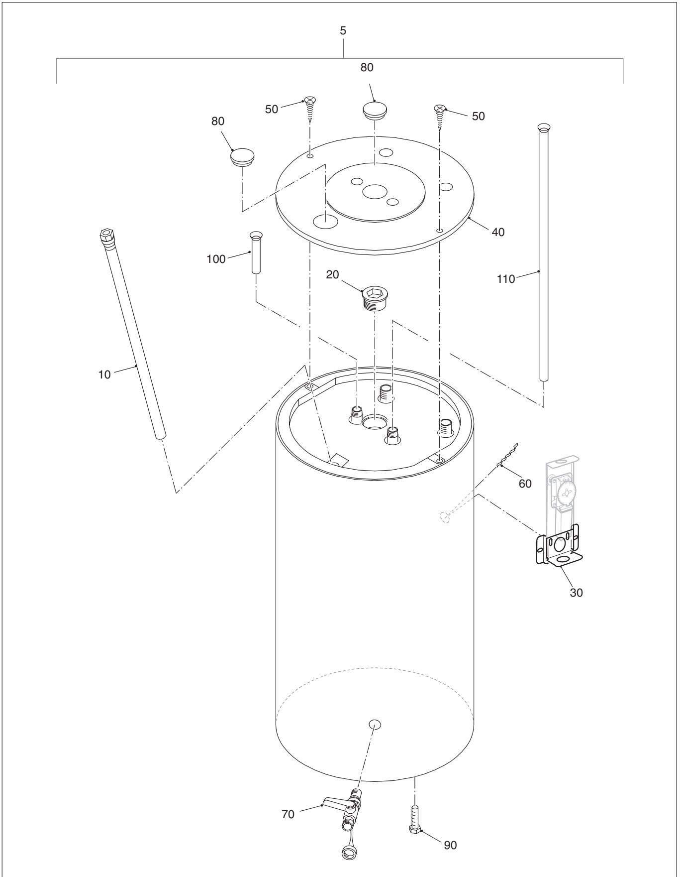
Fig. 12 Spare Parts for S120
