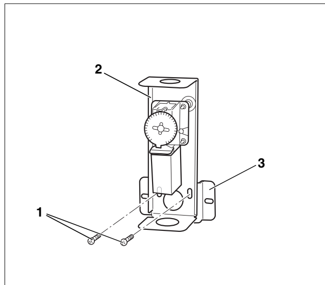
Fig. 8 Attaching bracket to aquastat
