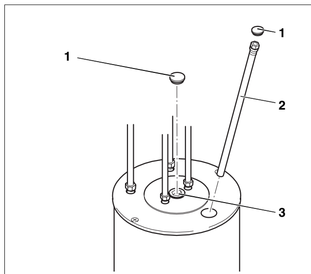
Fig. 10 Removal of magnesium anode rod
