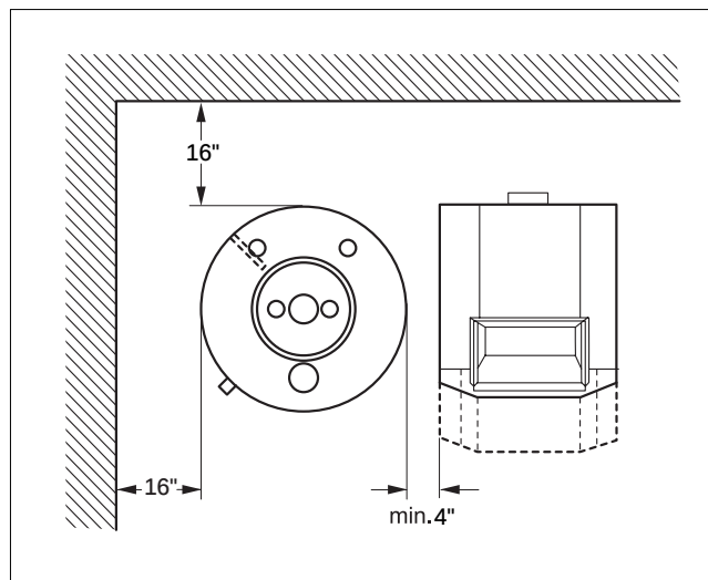
Fig. 1 Recommended clearance for installation and maintenance.
